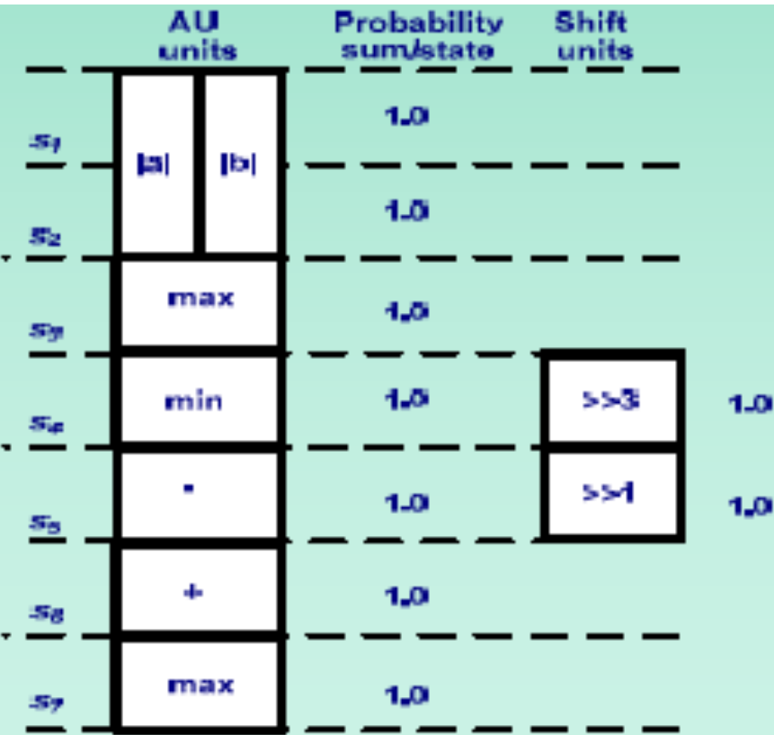
(c) Distribution graph after max, + and -, >>3 and >>1 were scheduled
