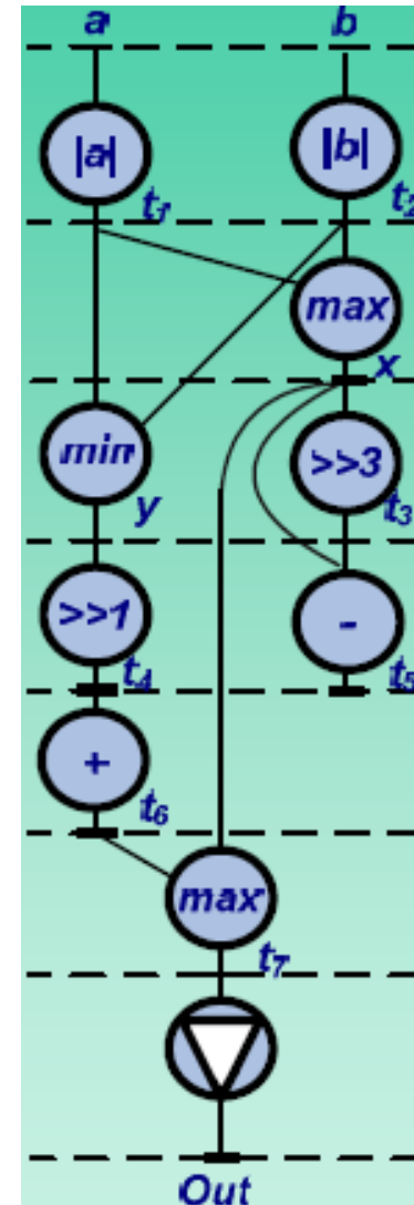
(b) ALAP schedule
